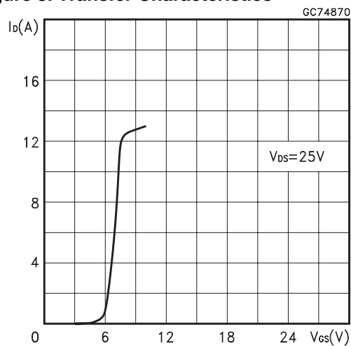
Figure 8. Transfer Characteristics
